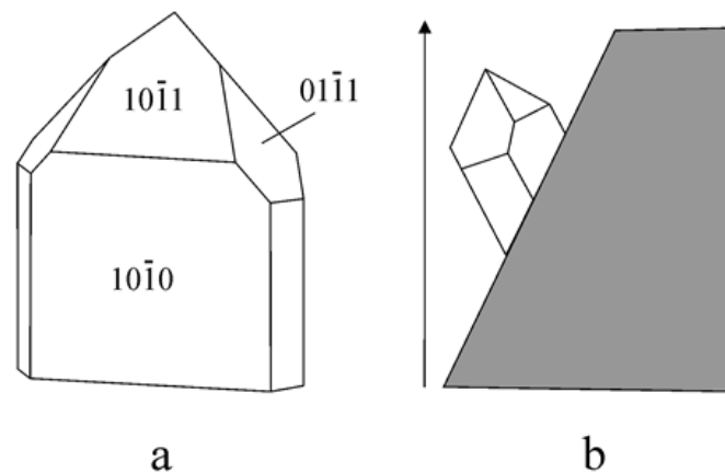
Fig. 1. Determining the direction of mineral-forming fluids from real quartz crystals [4]
